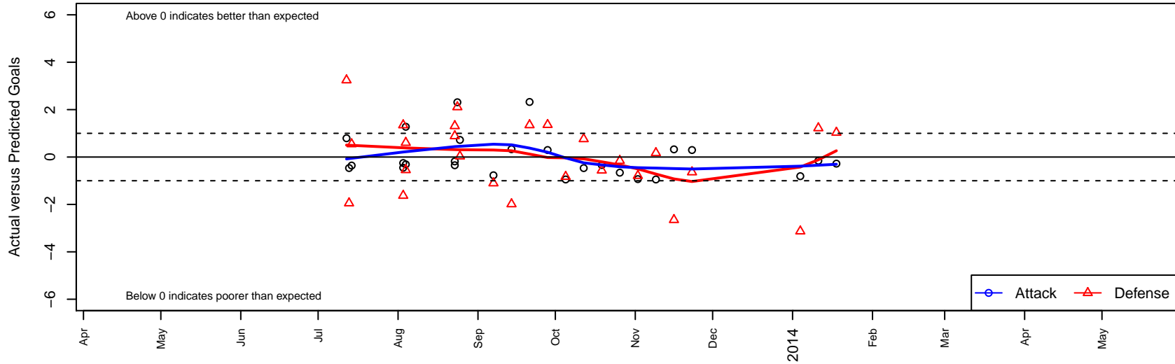
ISC Arsenal Red B01 Dots are actual minus expected GF (blue circles) and GA (red triangles). Blue line is smoothed change in attack strength. Red is smoothed change in defense strength.
